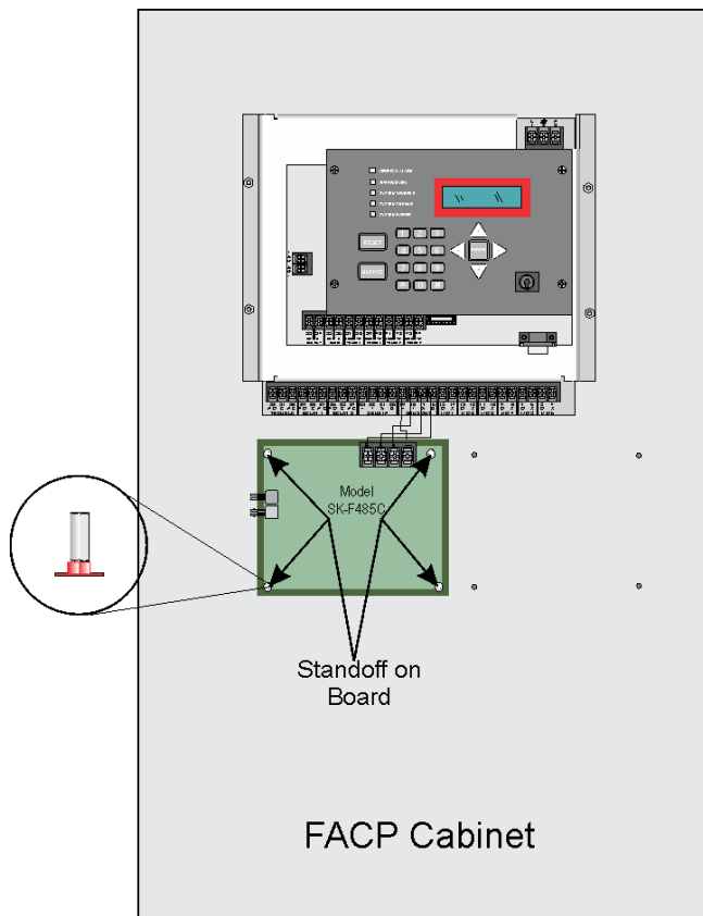
SK-F485C Mounting in FACP cabinet
