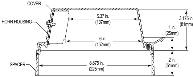
SIDE VIEW Models with Horn
