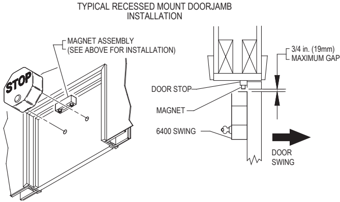
*Note: When mounting reed switch on door and the main unit on wall, wire service loop must be used. Figure 9
